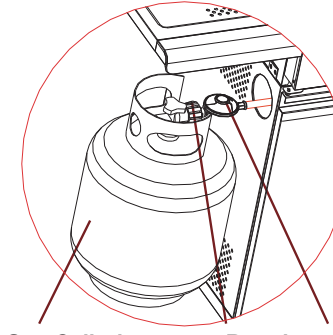
Gas Cylinder Regulator Hose Illustration for the connection of Gas Cylinder, Regulator and Hose. The regulator shall be approved by EN16129:2013.
